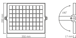
Solar panel
